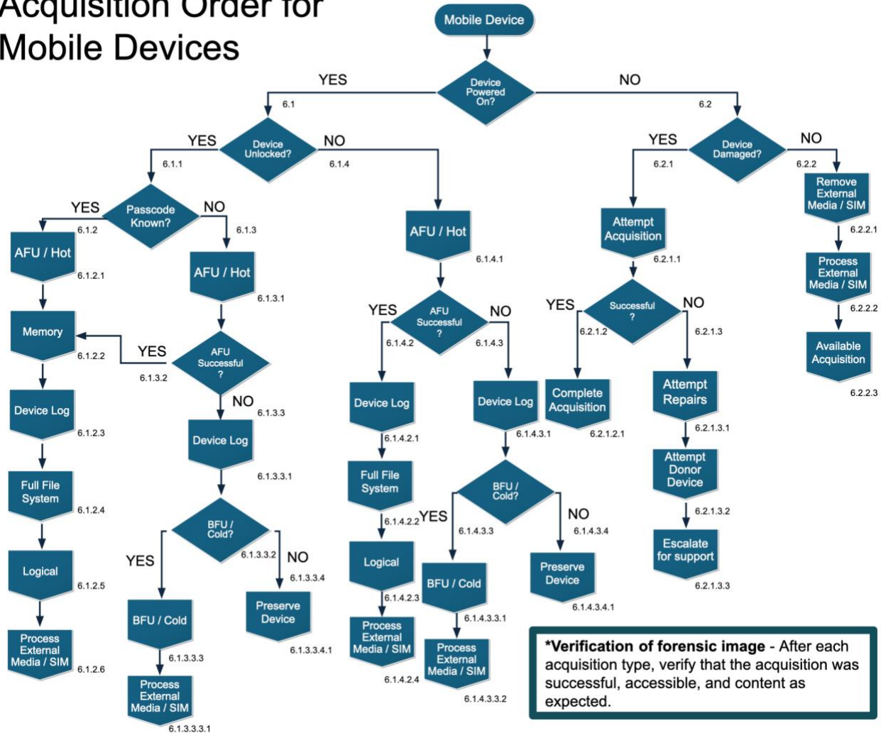
Figure 2. Acquisition Order for Mobile Devices. (Image Credit: SWGDE, 2025)
