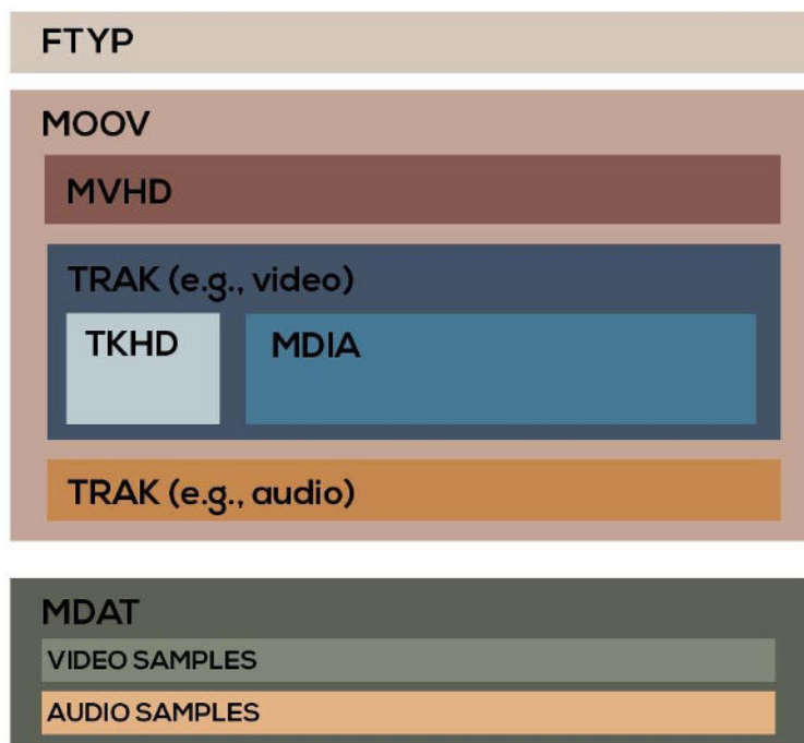
Figure 3: An illustration of some of the components that constitute an ISO Base Media File Format (e.g., MP4, MOV, 3GP) video file structure.
